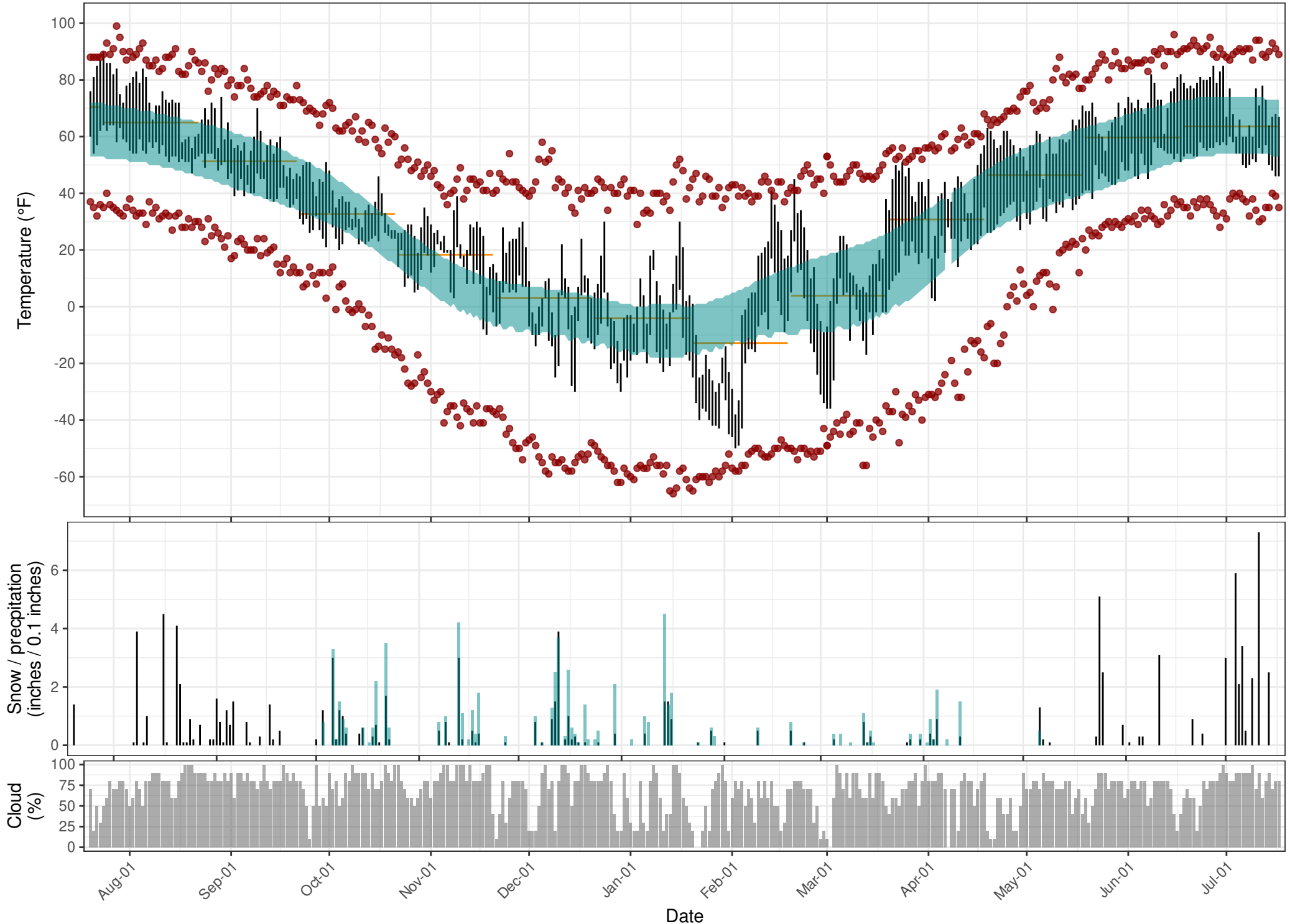
Daily temperature, precipitation and cloud cover, Fairbanks Airport (PAFA) 2023–2024
